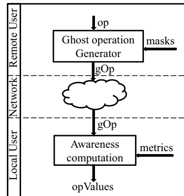
Figure 2. Generation of ghost operations, transmission through the network and computation of awareness after the operation's receipt.
