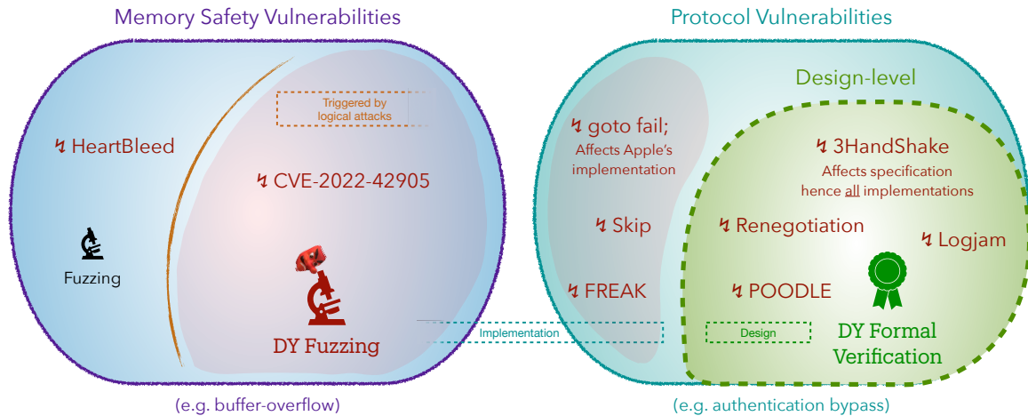
Figure 1.2.: Taxonomy of vulnerabilities in cryptographic protocol specifications and implementations, illustrated with TLS examples (detailed in Section 1.1). Design-level logical attacks (green area) exploit flaws in the protocol’s logic specification (e.g., Triple Handshake [Bha+14], POODLE [MDK14], Renegotiation [CVE09-3555], Logjam [Adr+15]) and are well-captured by formal verification. Logical attacks can also be introduced at the implementation level through bugs in the code. These can manifest as protocol vulnerabilities (such as the authentication bypass caused by Apple’s Goto Fail bug [CVE14-1266], or Skip/FREAK [Beu+15]) or as memory-safety vulnerabilities (e.g., CVE-2022-42905, see Part C). As we shall see, standard fuzzing targets non-logical memory-safety bugs (e.g., Heartbleed [Meh+14]), but misses the first three classes. The middle area in red highlights the blind spot of current software testing techniques.
