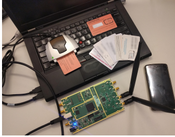
Figure 7.5.: Our experimental setup, showing a smartcard reader, USRP (left), set of commercial USIM cards, and a test phone.
