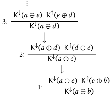
Figure 4.1.: Example 4.1.1: Infinite chain of deconstruction rules.
