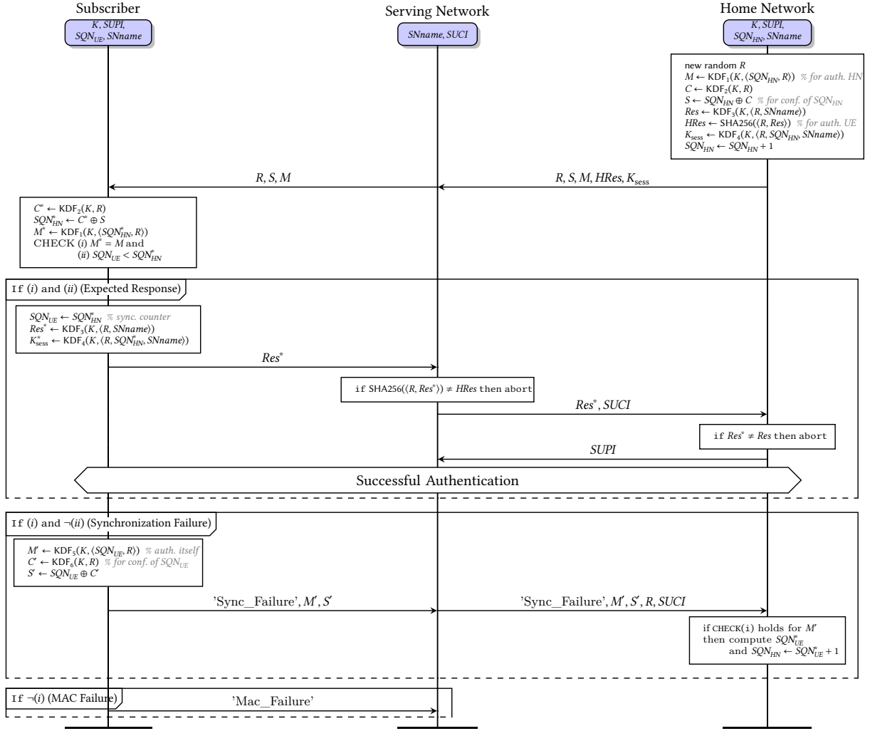
Figure 7.3.: The 5G AKA protocol, simplified presentation (continuing Figure 7.2)
