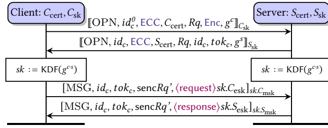
Figure 6.3.: (Re)Open Secure Channel (first two messages) and Channel Communications (last two) in (ECC + Enc). OPN is a header string. After the first two messages, client and server can derive a set of symmetric keys sk containing encryption keys C_{esk} , S_{esk} and HMAC keys C_{msk} , S_{msk} . The last two messages describe the channel protection of subsequent requests/responses payloads \langle \text{request} \rangle / \langle \text{response} \rangle (cf. Section 6.1.2.2).
