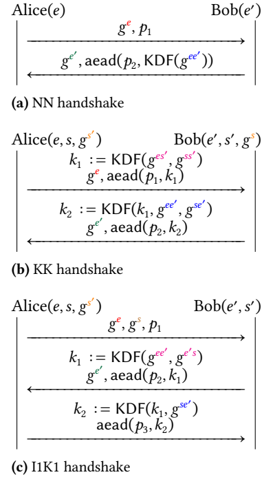
Figure 2.3.: Alice & Bob notation for the handshakes of Figure 2.2. e, e' (respectively s, s' ) are ephemeral (respectively static) private keys and the p_i are payloads exchanged during the handshake. In transport mode, payloads are encrypted with the last key material used in the handshake. For legibility, we omitted the associated data of AEAD encryptions, which roughly corresponds to the hash of all preceding sent messages along with the public keys in pre-messages.
