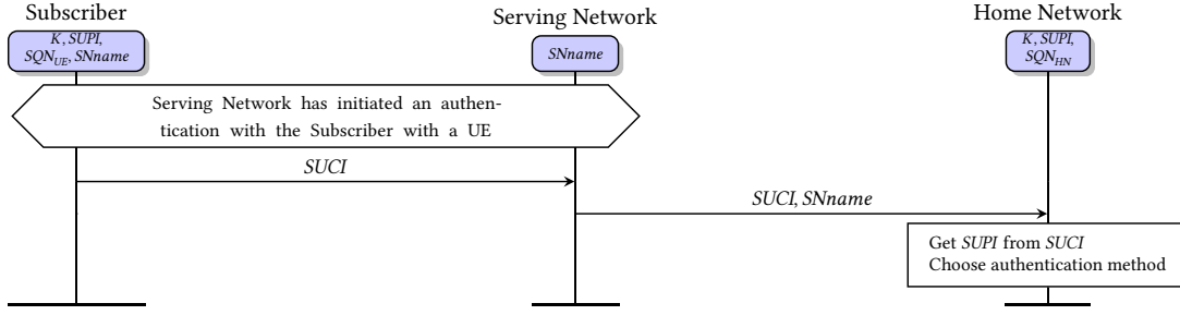
Figure 7.2.: Initiation of Authentication in 5G AKA. SUCI encrypts SUPI with HN 's public key to protect subscriber's identity.
