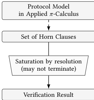
Figure 2.10.: PROVERIF’s verification workflow. \rightarrow : translation or process is sound & complete. \dashrightarrow : translation is sound only (over-approximation). The saturation procedure also takes the security property to verify as input.
