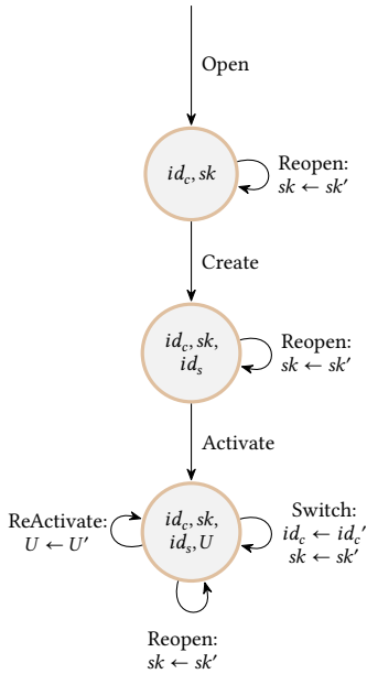
Figure 6.2.: Overview of the OPC UA state machine
