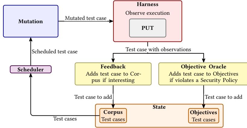
Figure 9.1: Generic fuzzer architecture (terminology based on LIBAFL [Fio+22]). The Scheduler picks a test case from the Corpus and the Mutation stage produces a mutated variant, which the Harness executes on the PUT while observing its execution. The resulting observations are analyzed by two components: the Feedback , which adds the test case to the Corpus when deemed interesting (e.g., new code coverage), and the Objective Oracle , which stores the test case in the Objectives when it violates a Security Policy (e.g., a crash or a memory error).
