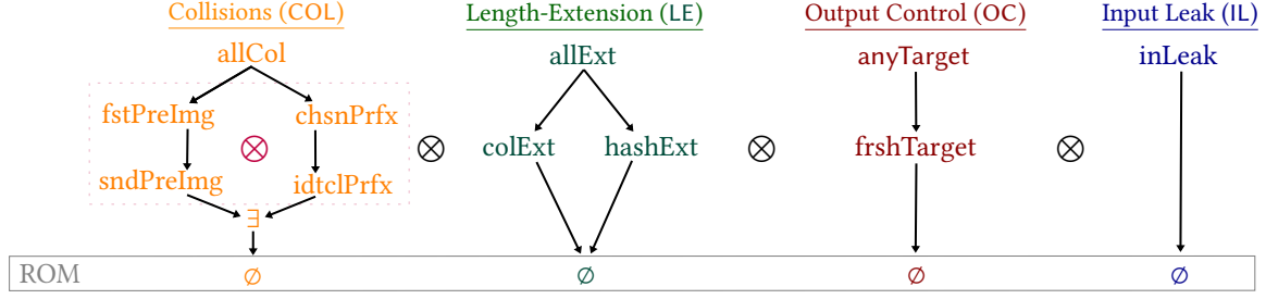
Figure 3.2.: Lattice of adversarial capabilities. An edge x \rightarrow y expresses that x is a stronger capability than y . Each column is a dimension described at the top. Capabilities from different dimensions can be combined into threat models, e.g., \{\text{idtclPrfx}, \text{allExt}\} . The minimal threat model is the empty one, \emptyset , which corresponds to the ROM.
