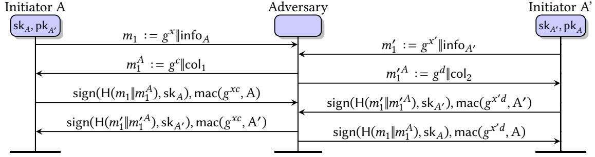
Figure 3.3.: The new CPC attack we found on Sigma'. \text{col}_i = \text{cp}_i(L_1, L_2) for i \in \{1, 2\} where L_1 := g^x || \text{info}_A || g^c and L_2 := g^{x'} || \text{info}_{A'} || g^d . Therefore H(m_1 || m_1^A) = H(m_1' || m_1'^A) so that the signatures of A 's and A' can be reused.
