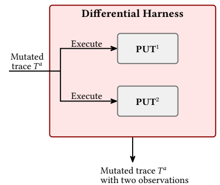
Figure 9.4.: Differential Harness Architecture for two PUTs. The execution of the trace on each PUT follows the same workflow as in Figure 9.2 but with two parallel executions and observations.
