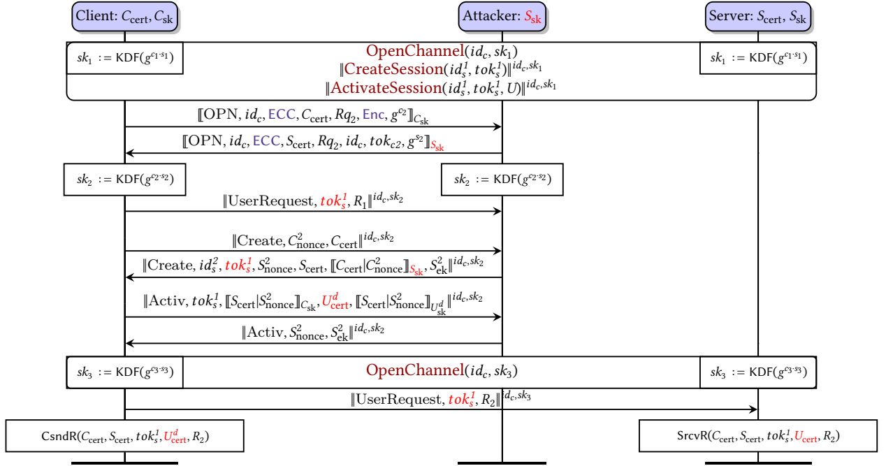
Figure 6.11.: Session confusion illustrated here with Mode = Enc, SecurityPolicy = ECC and SessionSecurity = SSec.
