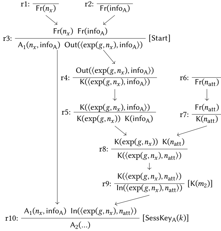
Figure 2.7.: Example execution of P_{Sigma'} \cup MD , where m_1 \triangleq \langle exp(g, n_x), info_A \rangle , m_2 \triangleq \langle exp(g, n_x), n_{att} \rangle , and k \triangleq exp(exp(g, n_x), n_x) . The arrows denote causal dependencies. In particular, these dependencies correspond to the edges D of the underlying dependency graph, where I \triangleq [r1, \dots, r10] . In this execution, the adversary intercepts the first initiator's message and replays the Diffie-Hellman share along with the adversarially-chosen nonce n_{att} (instead of info_B ). Rules r5 and r8 are instances of the projector \pi_1 (deconstruction) and the pairing operator \langle \cdot, \cdot \rangle (construction), respectively; r7 is the adversary-fresh rule that allows the adversary to generate fresh values. The trace of this execution is [Start, K(m_2), SessKey_A(k)] .
