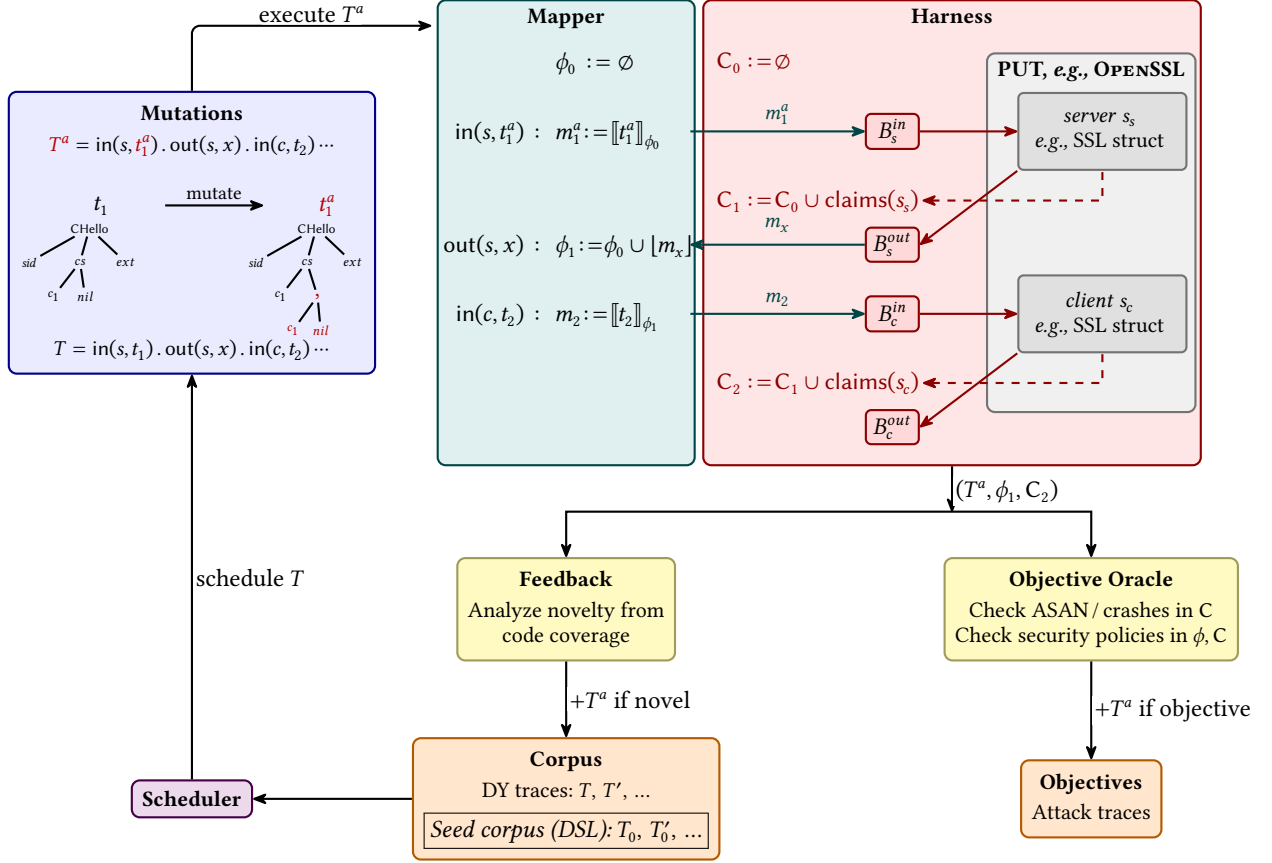
Figure 9.2.: Overview of the DY fuzzing loop (DY-specific instantiation of Figure 9.1). Starting from a Seed Corpus of symbolic DY traces, the Mutation stage applies term-level and action-level mutations to produce a new trace T^a . The Mapper concretizes each attacker term into a bitstring under the current attacker's state \phi (e.g., m_1^a = \llbracket t_1^a \rrbracket_{\phi_0} ) and, after the PUT responds, parses the output message to extend \phi . The Harness manages the PUT instances (here a server s_s and a client s_c , each with its own SSL struct) and uses input/output buffers B_s^{\text{in}}/B_s^{\text{out}} to exchange messages with them. Note that the same agents and their buffer pairs is reused across all protocol steps of a given trace (e.g., the same B_s^{\text{in}} is used for all messages inputs to the server s_s ), but are re-initialized before executing a new trace. After each action execution, claims C are extracted from the PUT internal state to capture security-relevant information (e.g., negotiated parameters). The Feedback component evaluates the novelty of the execution based on code coverage, while the Objective Oracle checks for memory errors (via ASAN) and for violations of DY security policies over \phi and C .
