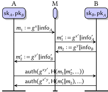
Figure 3.1: CPC attack on Sigma': an adversary M forges m'_1, m'_2 so that H(m_1 \| m'_2) = H(m'_1 \| m_2) , hijacking the session key g^{xy'} = g^{x'y} . Here, \text{auth}(k, h, \dots) denotes the signature and MAC exchange of Figure 2.1 using session key k and transcript hash h .
