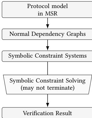
Figure 2.6.: TAMARIN's verification workflow. All steps ( \rightarrow ) are sound & complete. The constraint solving procedure also takes the negation of the security property to verify as input.
