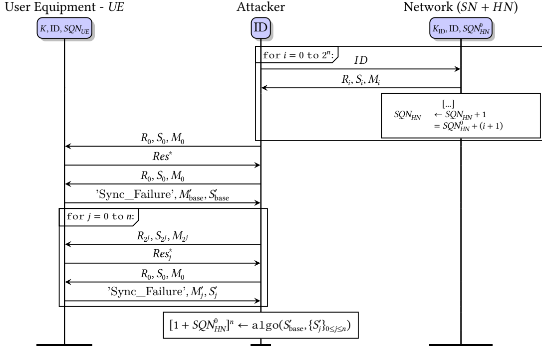
Figure 7.4.: Sequence Number Inference Attack. ID is a subscriber identifier, IMSI for 3G and 4G or an encryption thereof in 5G. SQN_{HN}^0 is the initial SQN for ID stored in the HN and [X]^n denotes the n least significant bits of X .
