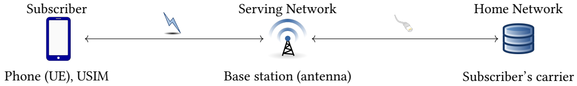
Figure 7.1.: Overall architecture in mobile communications: The subscriber uses their phone (UE), equipped with a USIM, to communicate with a base station run by the SN over an insecure wireless channel. The SN communicates with the subscriber's carrier (HN) on the right over an authenticated (wired) channel.
