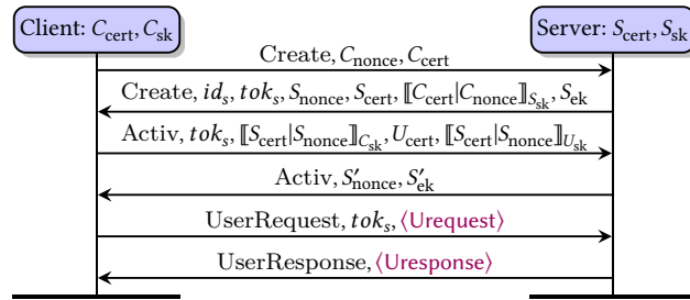
Figure 6.4.: Session creation (first two messages) and activation (third and fourth) and user requests/responses (last two) in (ECC + Enc + SSec + Cert). The session activation involves the user to produce the signature with U_{sk} . Create and Activ are header strings. The last two messages describe how user requests \langle \text{Urequest} \rangle and responses \langle \text{Uresponse} \rangle payloads, from the application layer, are wrapped in a session.
