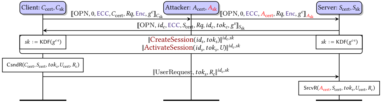
Figure 6.8.: Client impersonation attack when SecurityPolicy = ECC and SessionSecurity = SNoAA. Lack of agreement on the client during user Authentication is made possible by the same weakness that allows the KCI attack, i.e. , the lack of link to the client.
