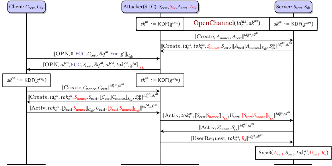
Figure 6.9.: KCI user impersonation attack when \text{SessionSecurity} = \text{SSec} (illustrated here when \text{SecurityPolicy} = \text{ECC} and \text{Mode} = \text{Enc} ). Values in a session between the attacker and the server (respectively client) are annotated with ^{as} (respectively ^{ca} ). We write \text{OpenChannel}(id_c^{as}, sk^{as}) for the channel open request and response messages with id_c^{as} identifier and keys sk^{as} .
