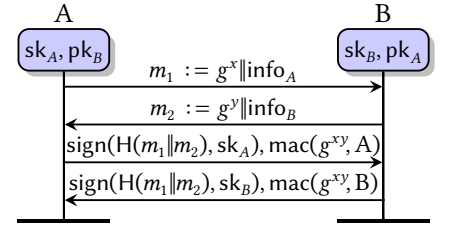
Figure 2.1.: The Sigma' protocol [BL16]. The operator \parallel denotes concatenation.
