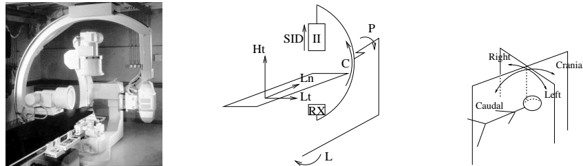
Figure 1: Angiography machine and anatomical angles
