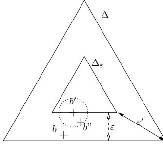
Figure 1: Simplices \Delta and \Delta_\epsilon , and the points b , b' and b'' .
