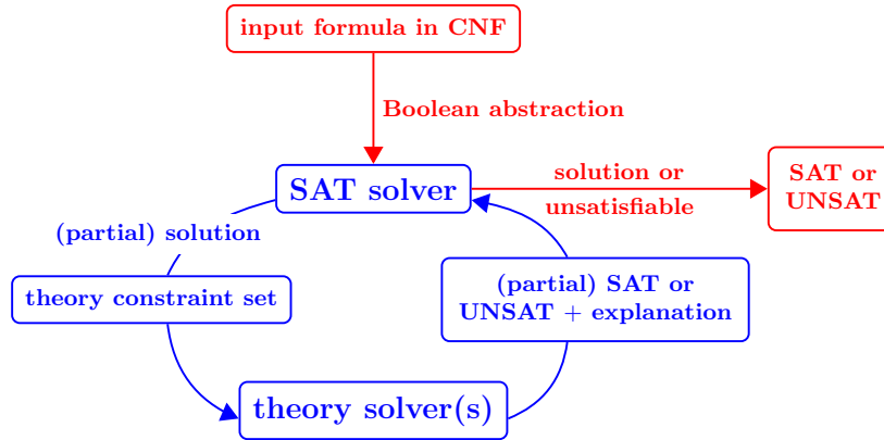
Fig. 2. The functioning of SMT solvers
