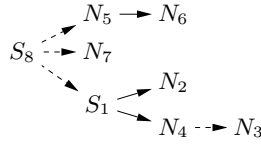
Fig. 6. The tree of rewrite and rooted Lambek edges for (S/N)/(N/N), N/N, N \vdash S
