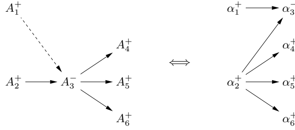
Fig. 4. The mapping between term graphs and LC-Graphs for neighbourhoods of negative vertices. The lambda variable \alpha_i corresponds to the atom occurrence A_i for 1 \leq i \leq 6 .
