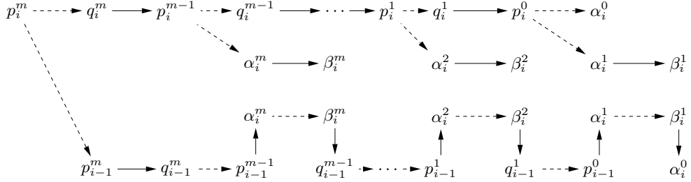
Fig. 9. Term graph for A_i \setminus B_i (for \alpha = a and \beta = b ) and C_i \setminus D_i (for \alpha = c and \beta = d )
