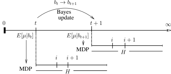
Figure 1. EXPLOIT-like algorithm. At each time step t , algorithm performs a Bayes update of the prior, and solves the MDP derived from the expected model of the belief.
